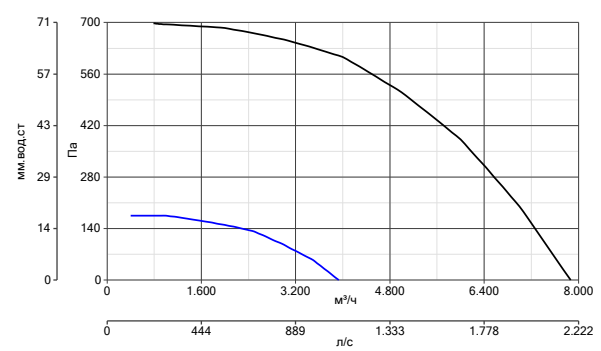
HEATMASTER F400 450 T4/T8 1.1/0.18KW
