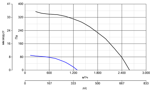
HEATMASTER F400 400 T4/T8 0.75/0.12KW
