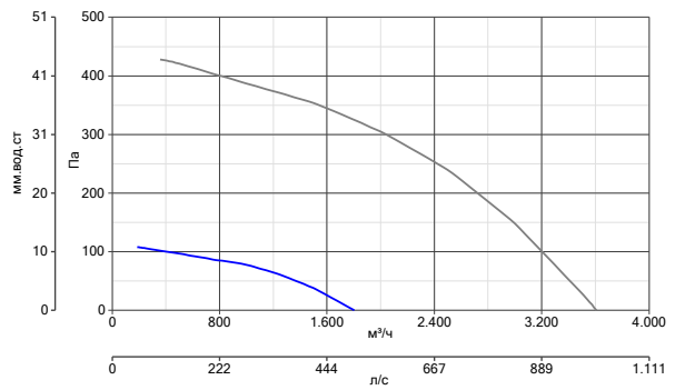
HEATMASTER F400 450 T4/T8 1.1/0.18KW
