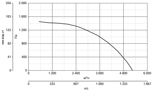
HEATMASTER F400 315 T4 0.25KW
